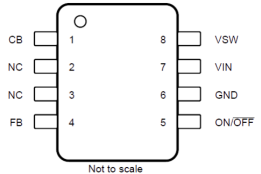
Top View SOP-8
