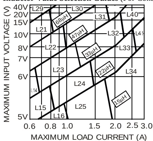
Figure 4. AP1501-3.3
