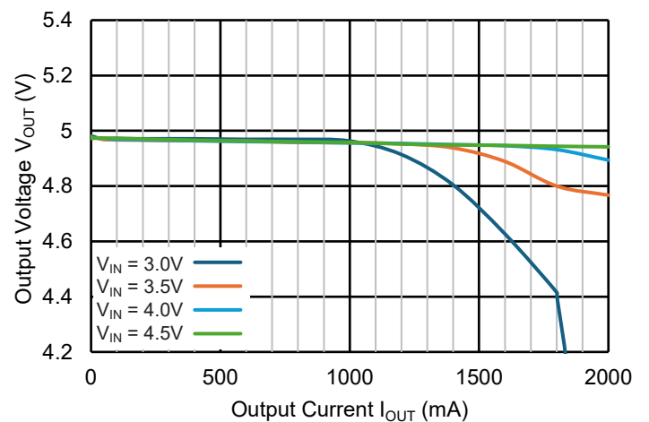
Load Regulation
