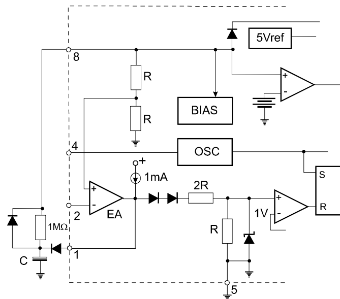
Figure 8. Soft-Start Circuit
