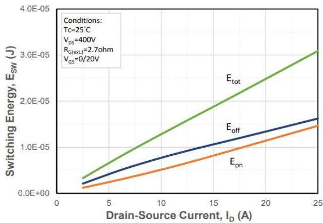
Figure 17. Clamped Inductive Switching Energy vs. Drain Current
