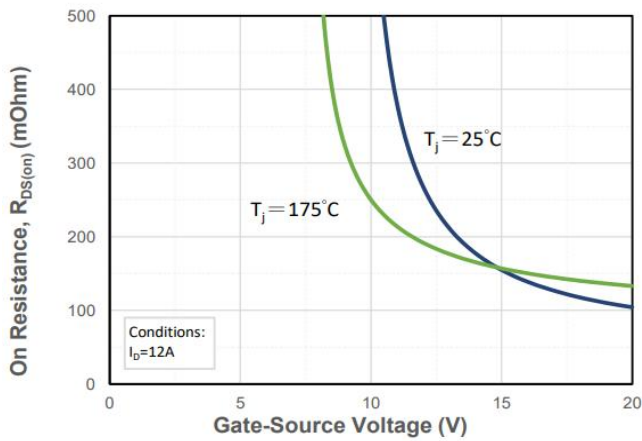
Figure 5. On-resistance vs. gate voltage for various T_J
