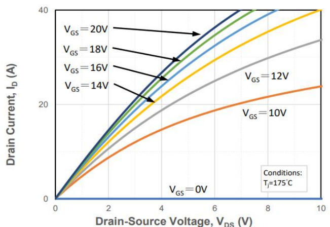
Figure2. Output Characteristics T_j = 175^\circ\text{C}
