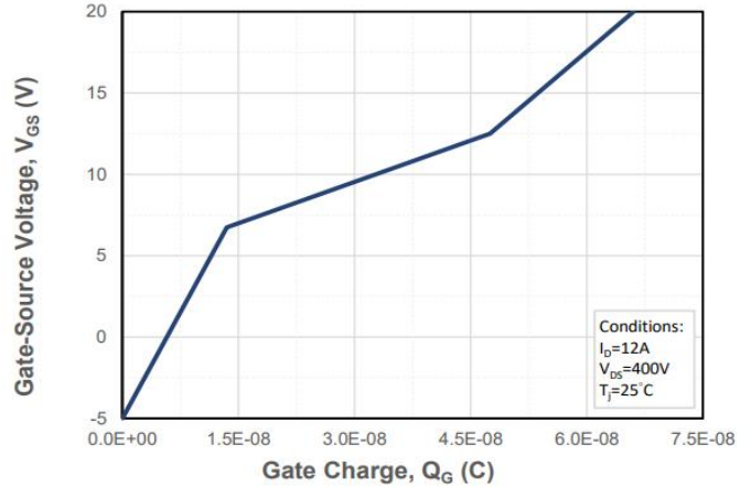
Figure 16. Gate Charge Characteristics
