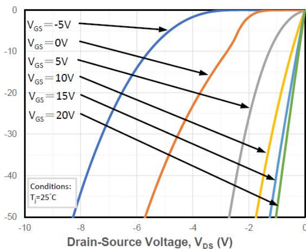
Figure 8. Reverse Output Characteristics at T_J = 25^\circ\text{C}
