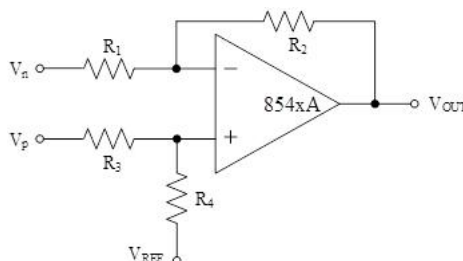
Figure 5 Differential Amplifier
