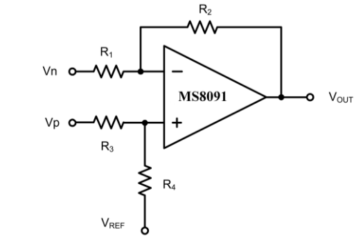
Figure 3. Differential Amplifier
