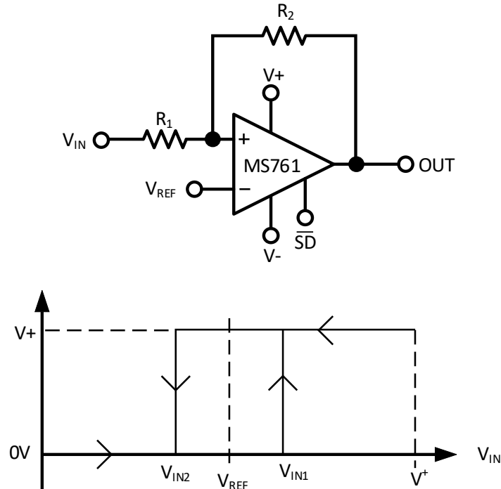
Figure 2. Non-inverting Comparator Circuit
