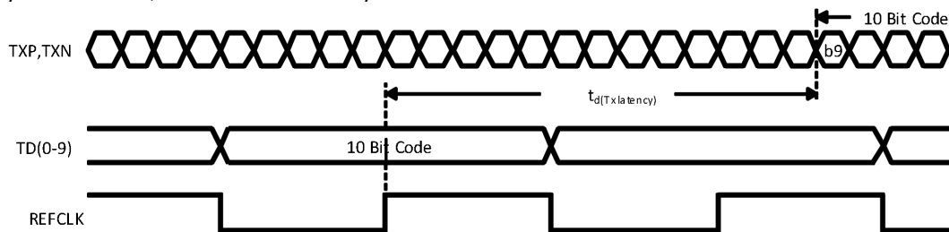
Figure 4. Transmit Latency in Full-rate Mode
