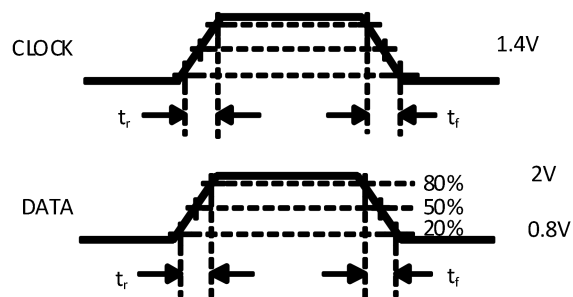
Figure 3. Valid Level of TTL I/O Data at AC Measurement
