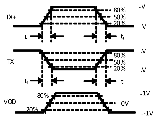
Figure 1. Definitions of Output Differential Signal and Common-mode Voltage
