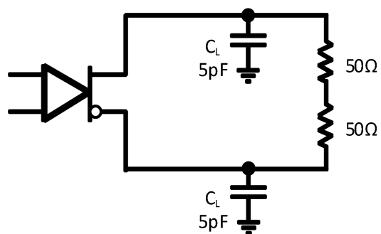
Figure 2. Setting of Transmitter Output Terminal
