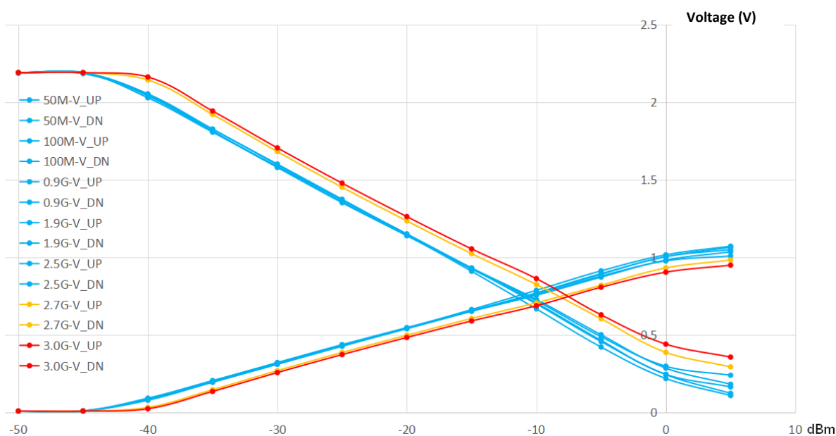
The Relationship between Input Signal Power, Input Signal Frequency, V_UP and V_DN in Typical Conditions
