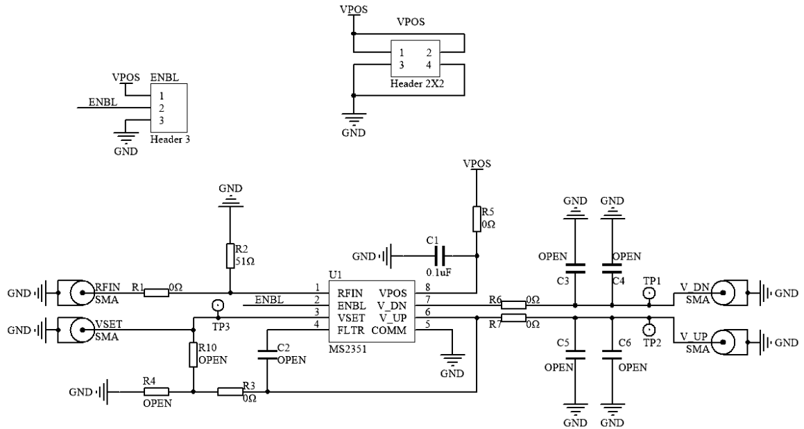
Figure 6. The MS2351 Evaluation Board
