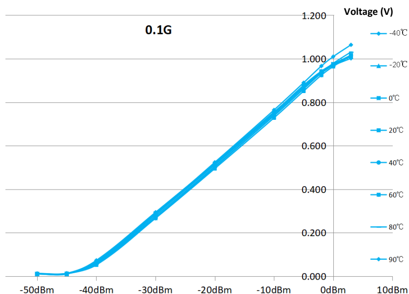
The Relationship between Input Signal Power and Output Voltage V_UP in 3.3V, 0.1GHz under Different Temperatures
