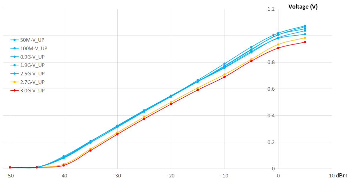
The Relationship between Input Signal Power, Input Signal Frequency and V_UP in Typical Conditions
