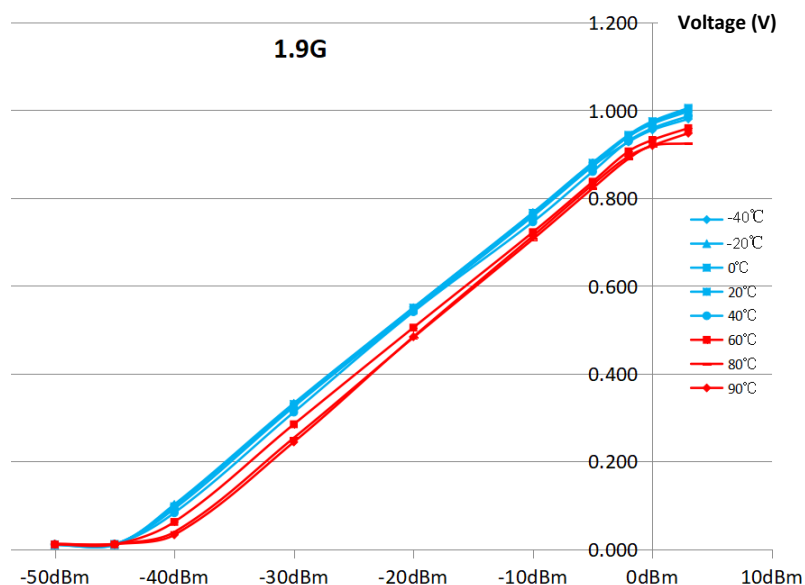
The Relationship between Input Signal Power and Output Voltage V_UP in 3.3V, 1.9GHz under Different Temperatures
