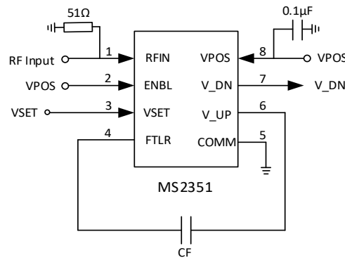
Figure 2. Control Mode
