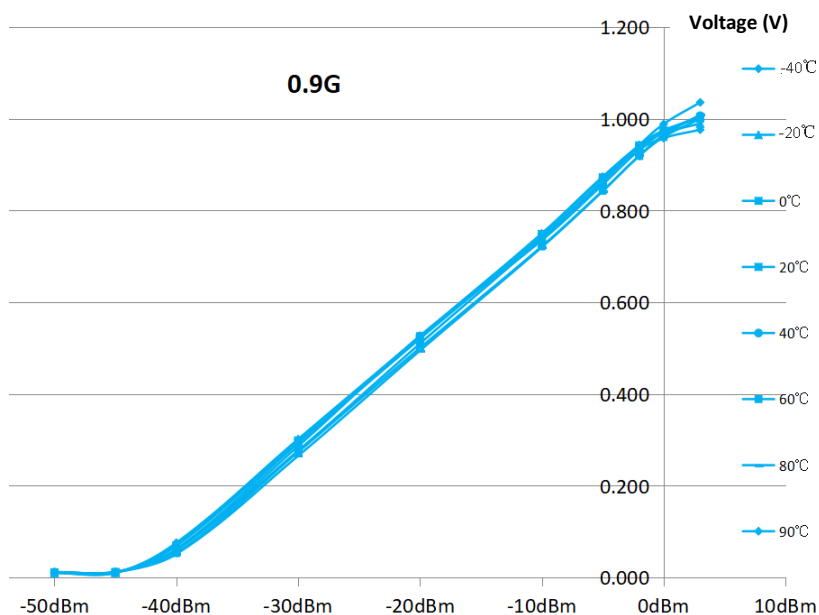
The Relationship between Input Signal Power and Output Voltage V_UP in 3.3V, 0.9GHz under Different Temperatures
