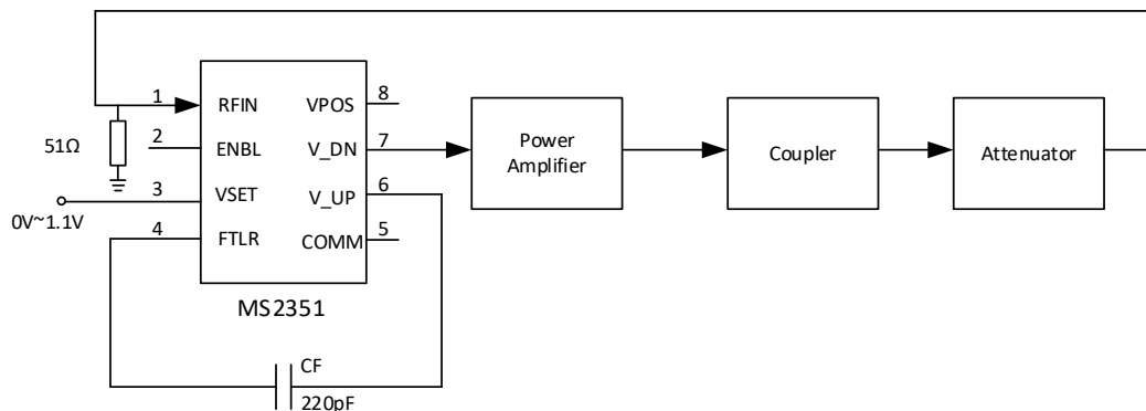
Figure 3. Typical Application in Control Mode
