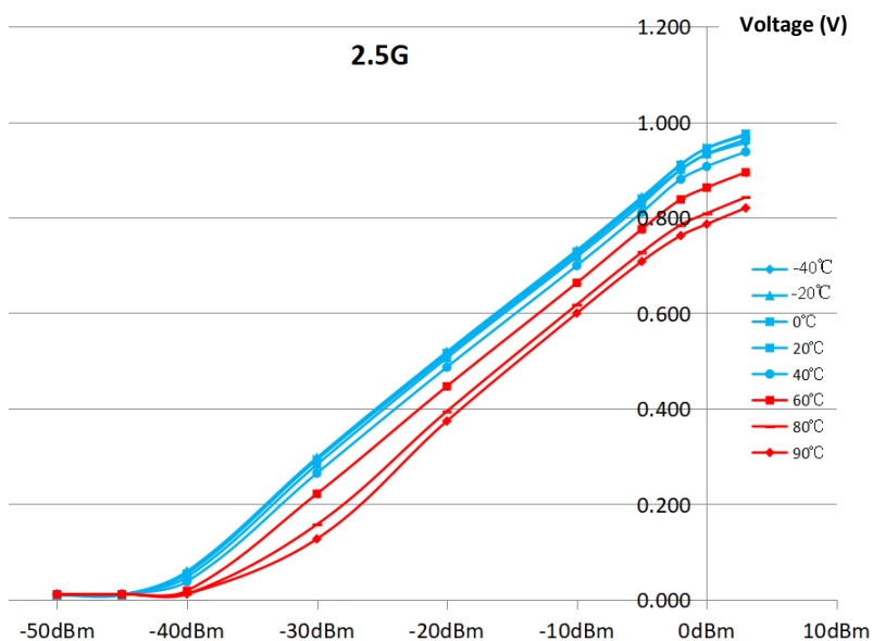
The Relationship between Input Signal Power and Output Voltage V_UP in 3.3V, 2.5GHz under Different Temperatures
