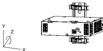
Rotate the installation position (0° Z-Axis)
