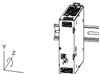
Rotate the installation position (90° Z-Axis)
