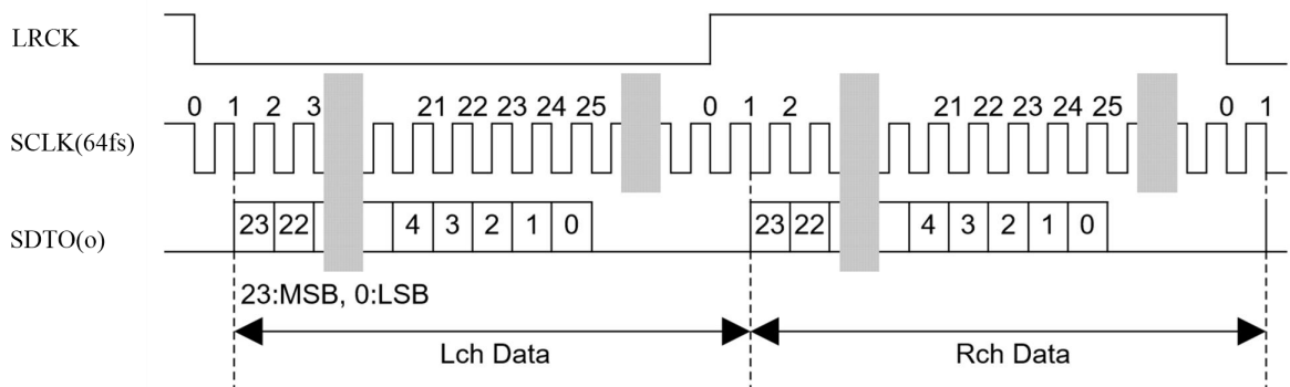
Figure 2. Mode 1 Timing
