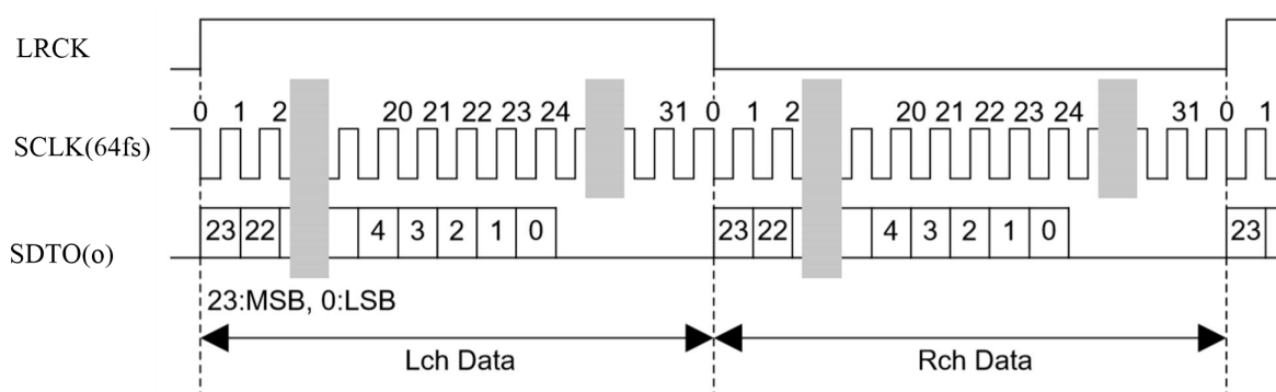
Figure 1. Mode 0 Timing
