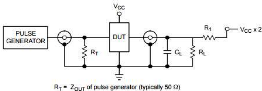
Figure 4. Test Circuit
