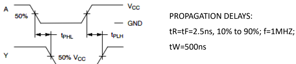
Figure3. Switch Waveform
