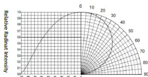
Relative Radiant Intensity vs. Angular Displacement
