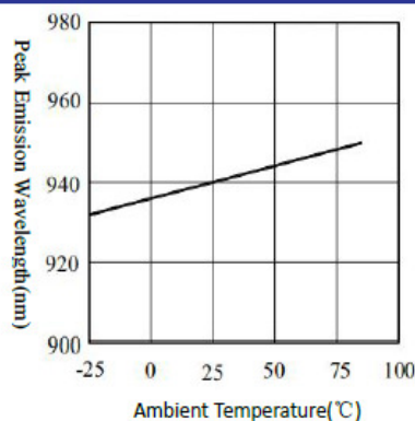
Peak Emission Wavelength vs. Ambient Temperature
