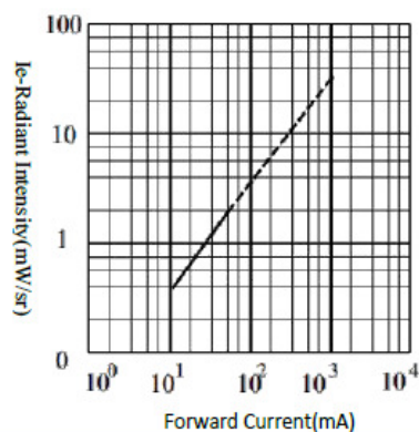
Radiant Intensity vs. Forward Current
