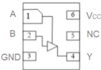
DFN6
