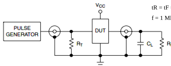
Figure 4. Test Circuit
