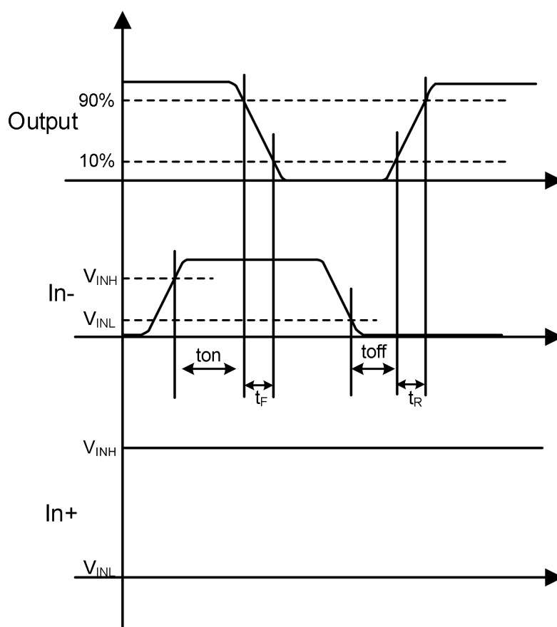
Figure 2 Input-Output waveform(inverting)
